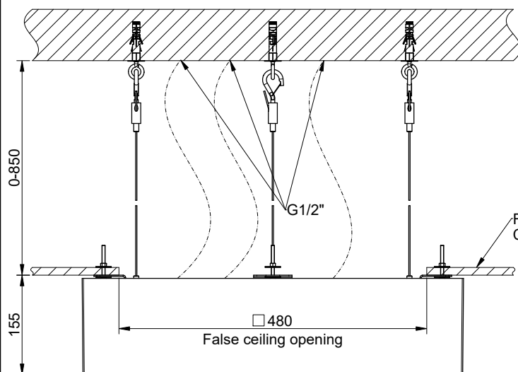
INSTALLATION MODE 1
