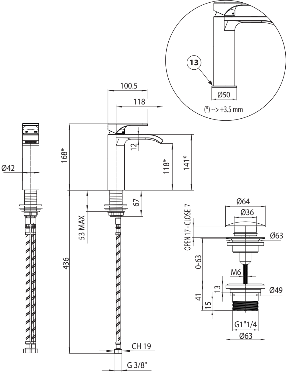
E89608 - Middle size basin mixer
