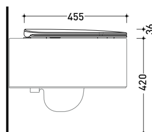
art. AS118G vista laterale / lateral view
