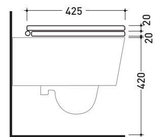
art. 5064 vista laterale / lateral view
