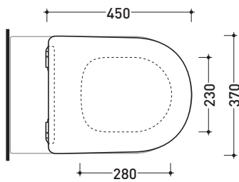
art. LK117 - LK117G - LK117RG vista zenitale / zenital view
